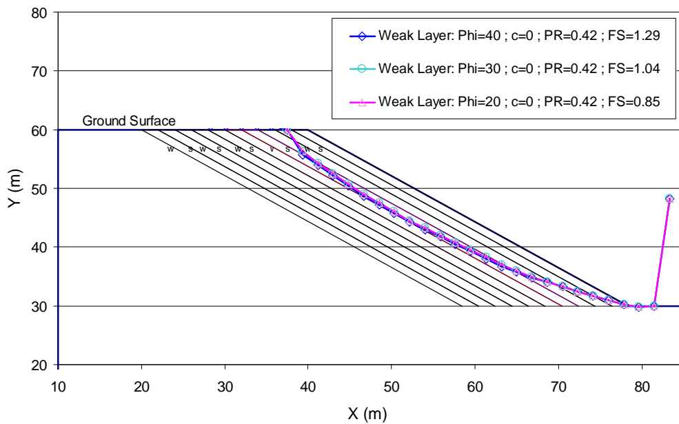
Figure 3: Effect of varying the angle of internal friction when Poisson's Ratio is equal to 0.42. Slope angle is 38 degrees.
