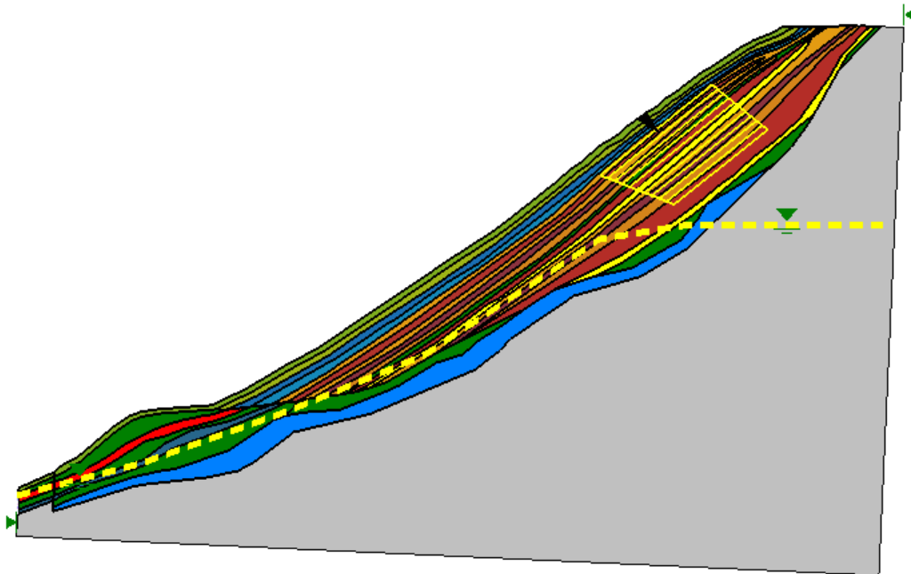
Figure 9: Level 3 water level
