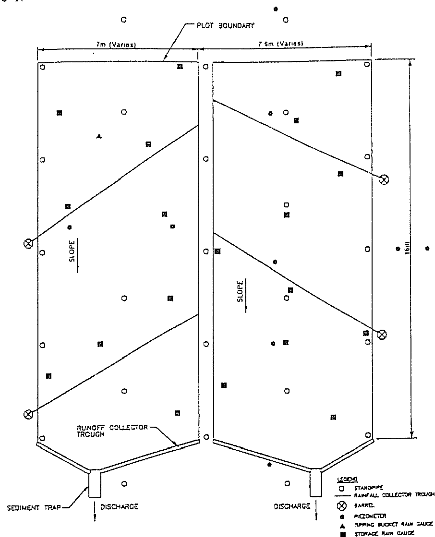
Figure 1: Rainfall Simulator and Instrumentation Layout
