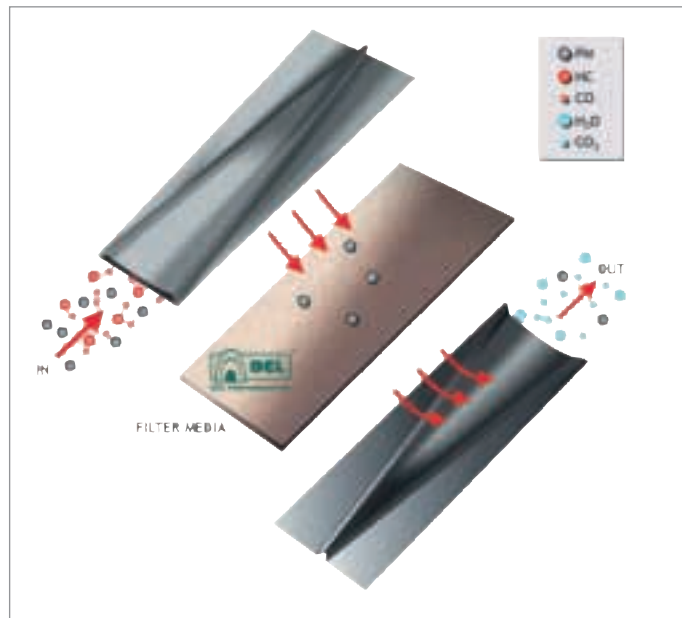
DCL's MINE-X Flow-Through Filter provides effective removal of DPM and lower back pressure than conventional wall-flow particulate filters
