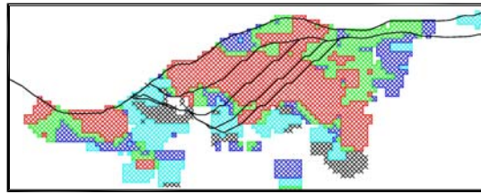
• Block Model Section Showing Extraction Sequences
