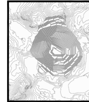
• Open Pit Phase Design With Topography
